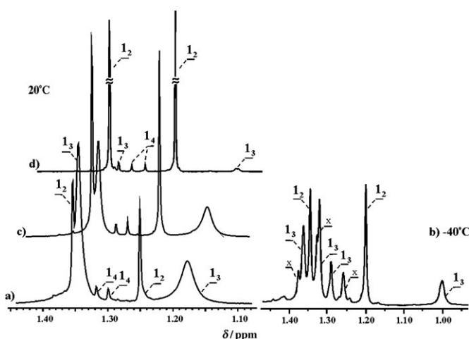
Figure 2. ^1\text{H} NMR spectra (in [\text{D}_8]\text{toluene} ) of a) freshly dissolved 1 at 20^{\circ}\text{C} , b) at -40^{\circ}\text{C} , c) after 20 min at 20^{\circ}\text{C} , and d) after 1.5 h at 20^{\circ}\text{C} .
